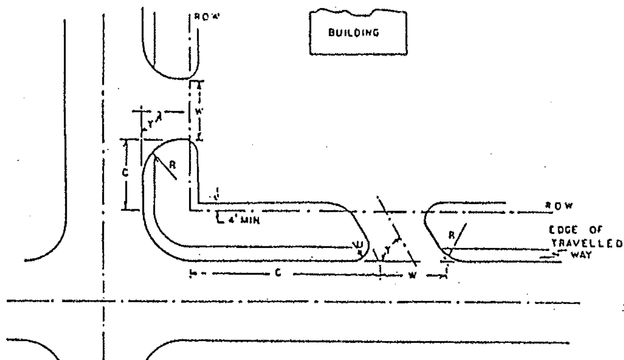
FIGURE 3. DRIVEWAYS FOR CORNER INSTALLATIONS—DIAGRAMMATIC
