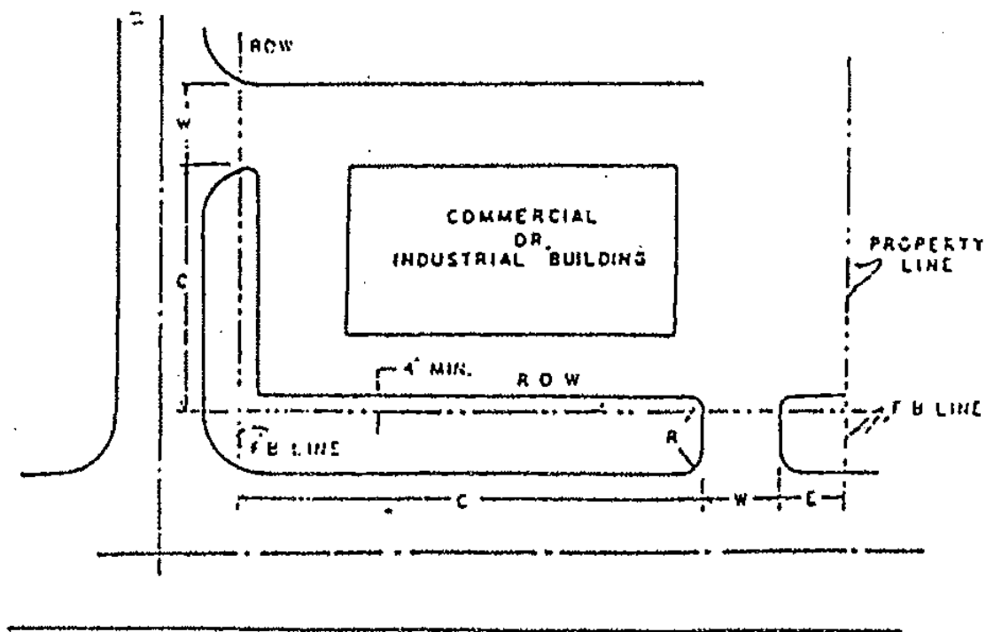
FIGURE 4. DRIVEWAYS TO A CORNER COMMERCIAL ESTABLISHMENT
