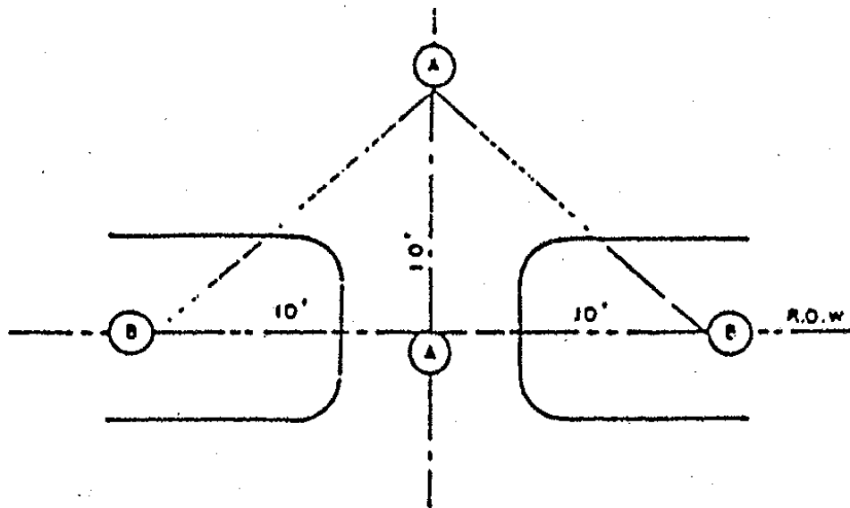
FIGURE 5B. VISIBILITY CLEARANCE (RESIDENTIAL)
