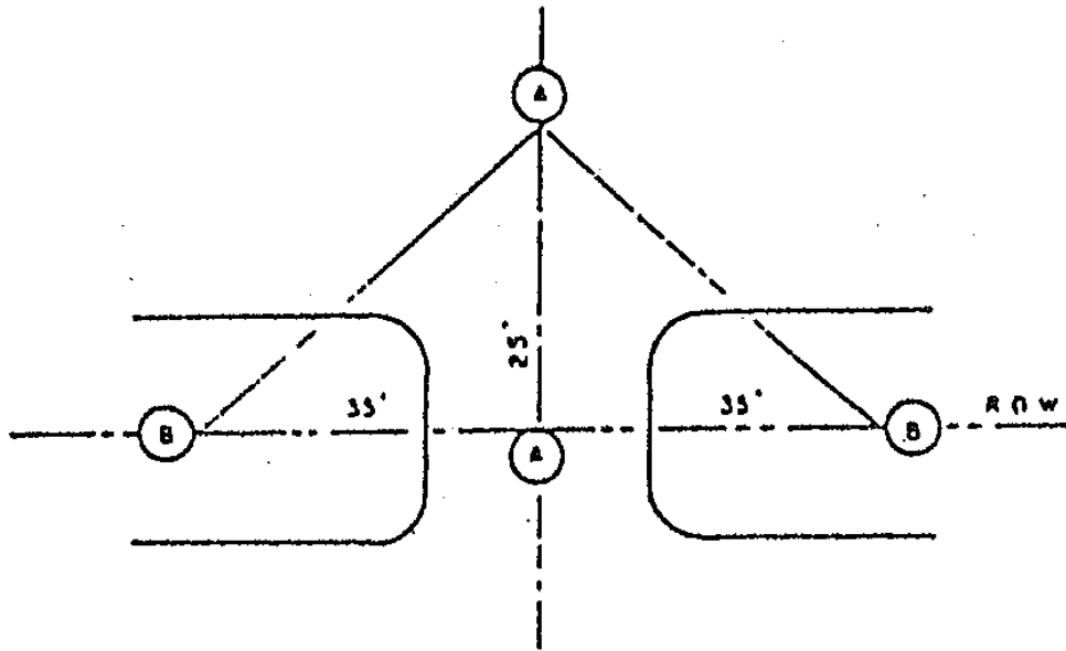
FIGURE 5A. VISIBILITY CLEARANCE (NON-RESIDENTIAL)
